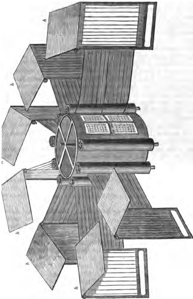
APPLEGATH'S "TIMES" VERTICAL PRINTING MACHINE. (10,000 sheets per hour.)
